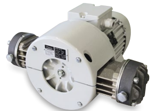
Compact version HAUG.Cygnus integrated in SPX-Delair dryers for compressed air in radar-systems on Navy ships.
